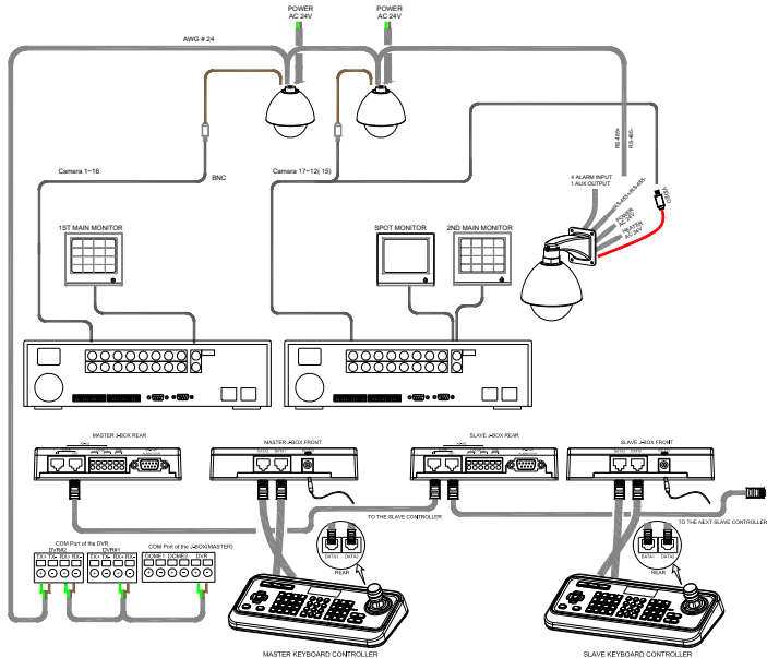
Figure 5 – Two DVR with Slave Controller
